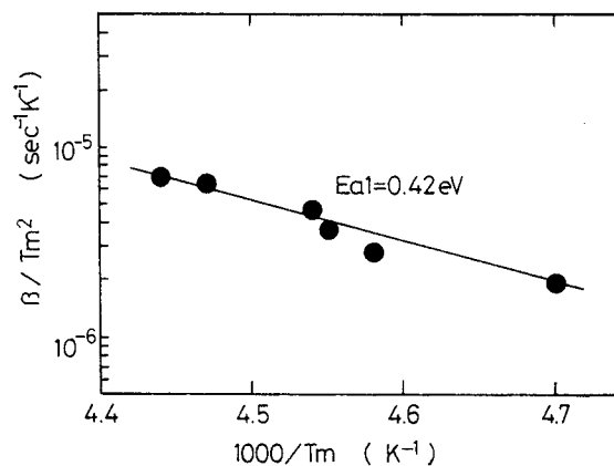
FIG. 5. \ln \beta/T_m^2 vs 1000/T_m . T_m is the temperature corresponding to a peak current for a given TSC curve with a heating rate ( \beta ).
